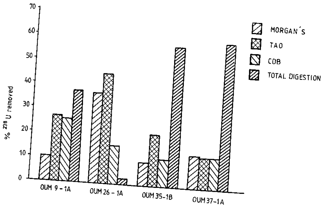
Figure 2-1. The percentage of total U removed by a particular extractant representing a particular phase(s), i.e. minus the uranium removed by the previous extractant.
