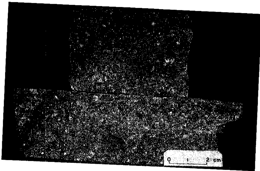
PLATE 3:9-2. Reduced medium-grained porphyritic phonolite with massive structures. The dark seams in the left hand corners of the drillcores are hydrothermally altered fractures mineralised with microcrystalline pyrite.
