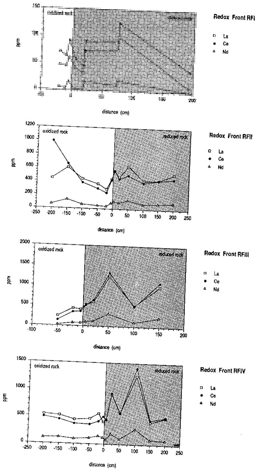
Figure 64. Distribution of LREEs across the redox fronts (data by XRF). RFI in a mineralised dense phonolite; RFII in a breccia; RFIII in a dense leucocratic phonolite; RFIV in a porous cpx-bearing phonolite.
