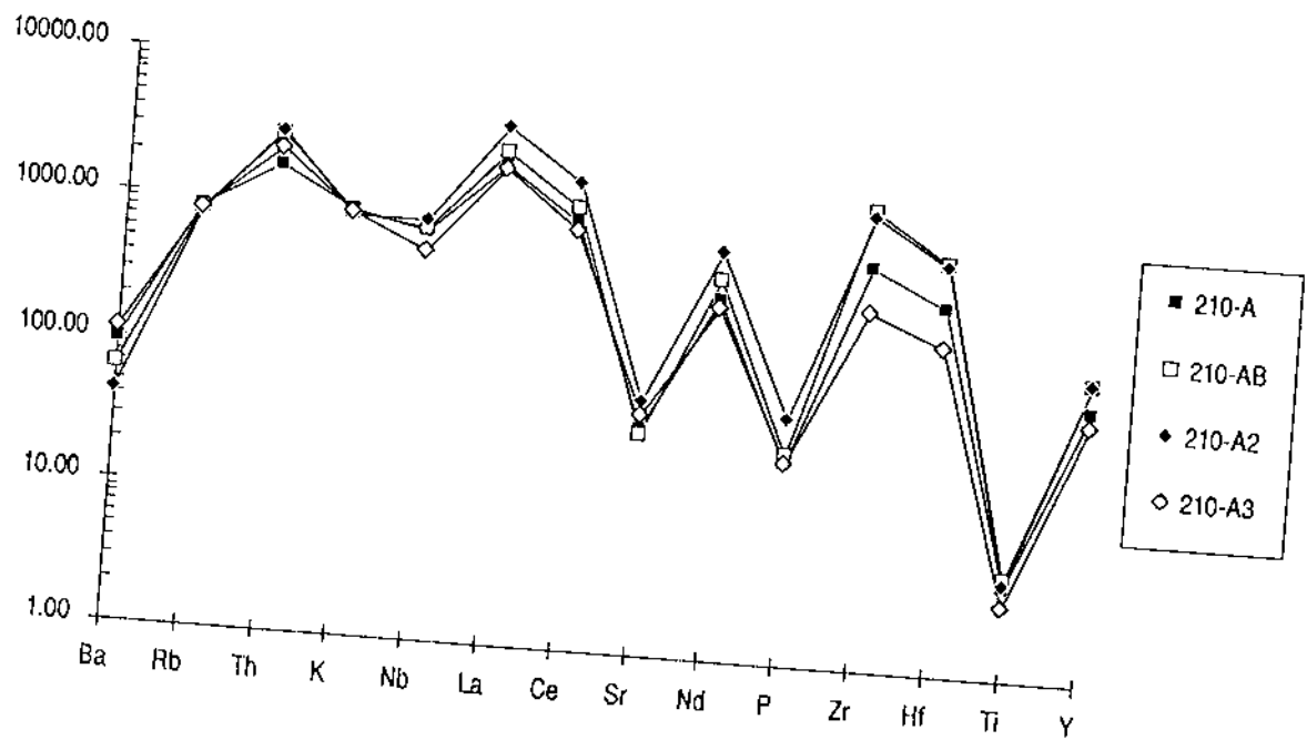
Figure 37. Incompatible elements normalised to chondrite and primitive mantle of the highly mineralised breccias at 210 m from borehole F4 (normalisation factors from Thompson, 1982).
