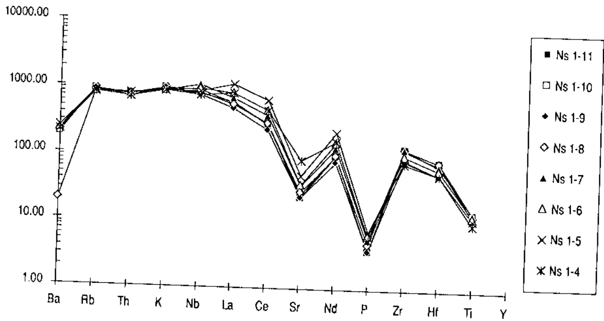
Figure 23. Incompatible elements normalised to chondrite and primitive mantle for hydrothermally altered, reduced nepheline syenite xenolith at 353 m depth from borehole F4; samples Ns 1-4 to 11 (normalisation factors from Thompson, 1982).
