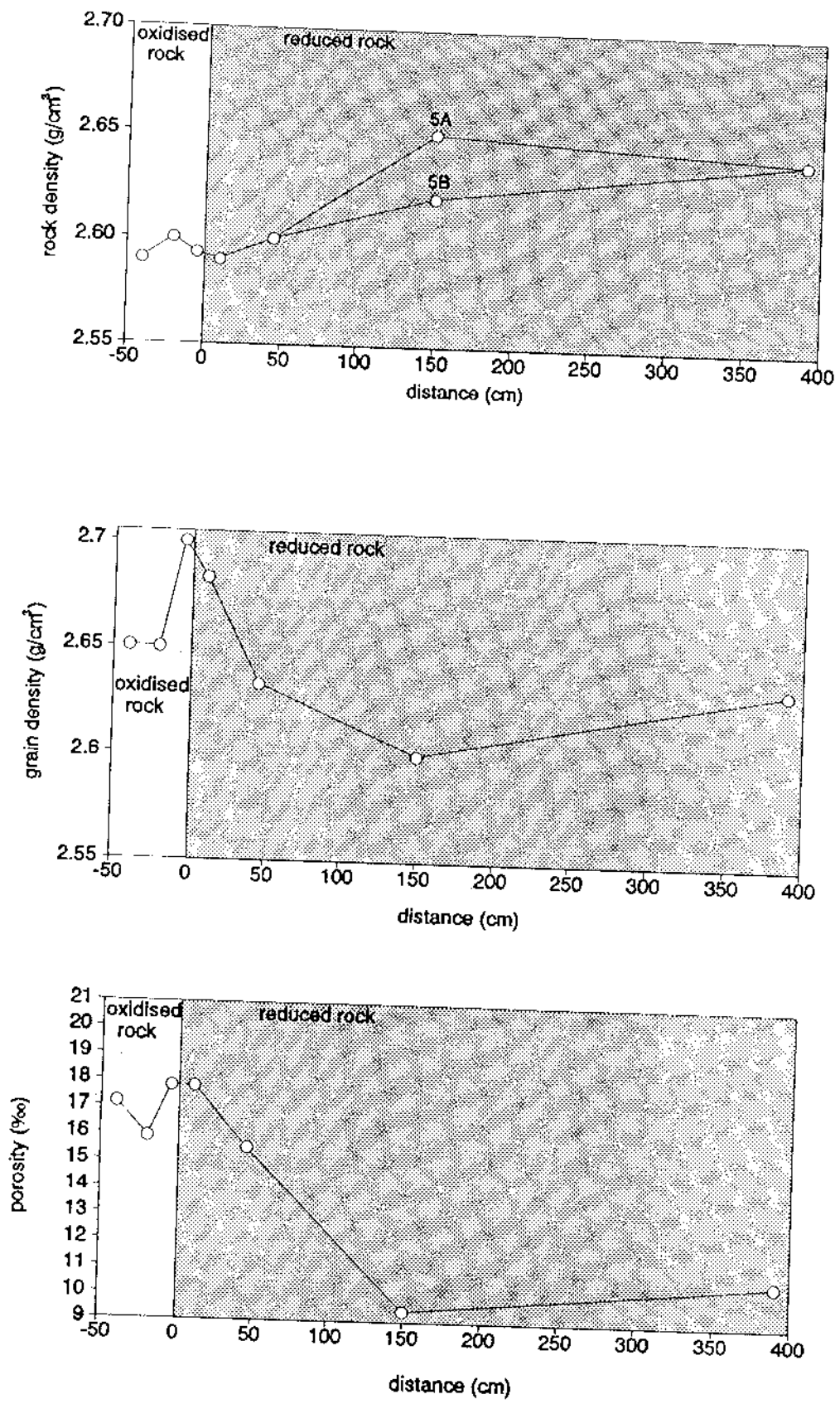
Figure 6-2. RFI redox front: distribution of rock physical properties.
