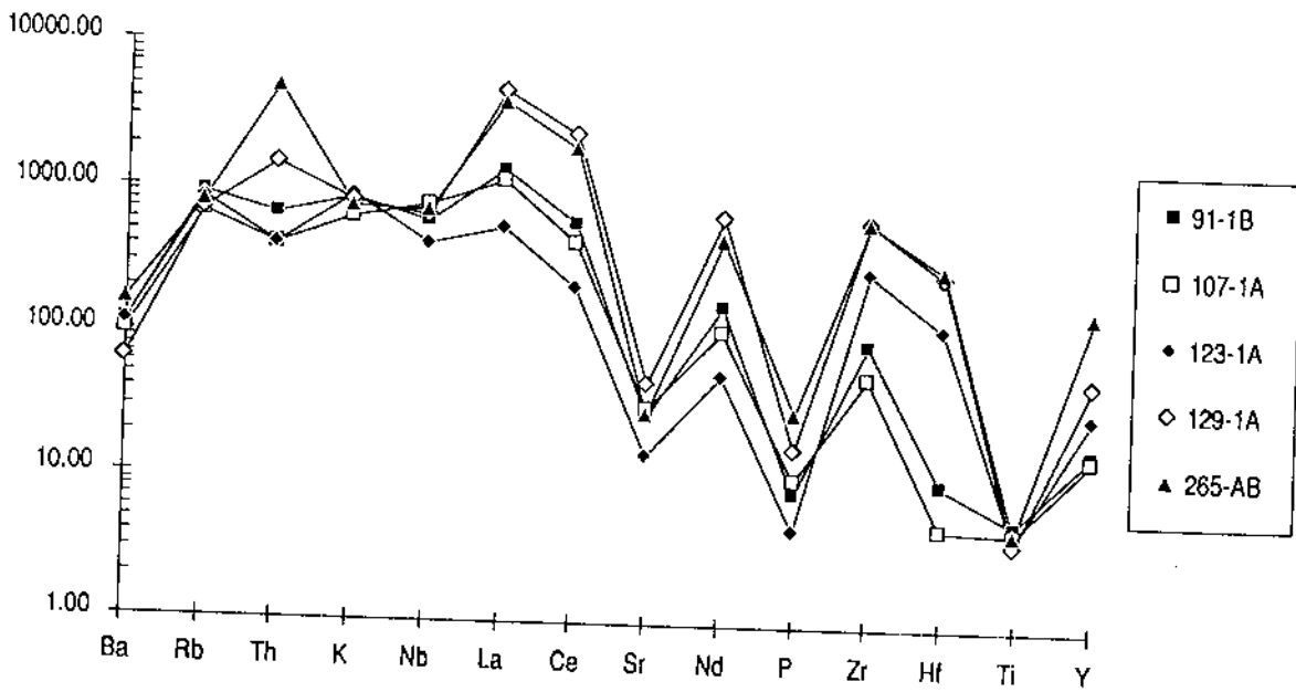
Figure 21. Incompatible elements normalised to chondrite and primitive mantle for hydrothermally altered, reduced nepheline syenite xenoliths from borehole F4, (normalisation factors from Thompson, 1982).
