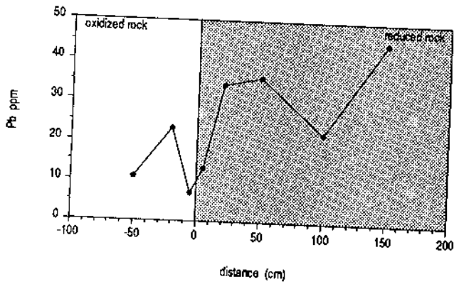
Redox Front RFIII
