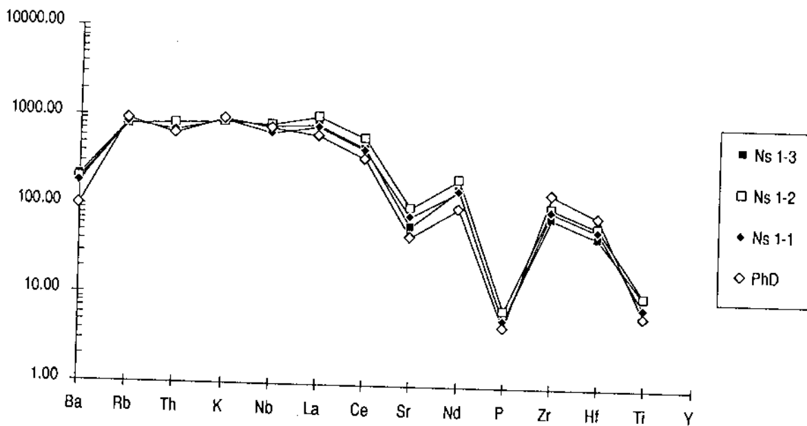
Figure 22. Incompatible elements normalised to chondrite and primitive mantle for hydrothermally altered, reduced nepheline syenite xenolith at 353 m depth from borehole F4 (samples Ns1-1 to 3) and the phonolitic dyke (sample PhD), (normalisation factors from Thompson, 1982).
