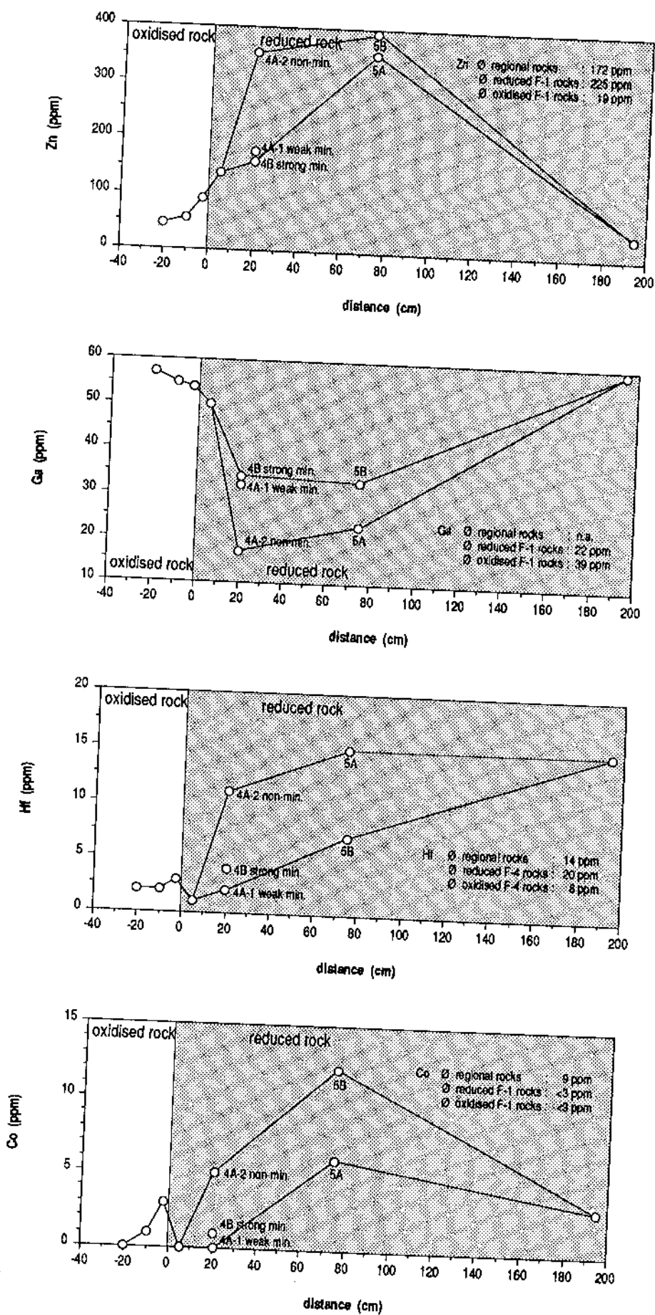
Figure 6-11. RFI redox front: geochemical distribution of Zn, Ga, Hf and Co.
