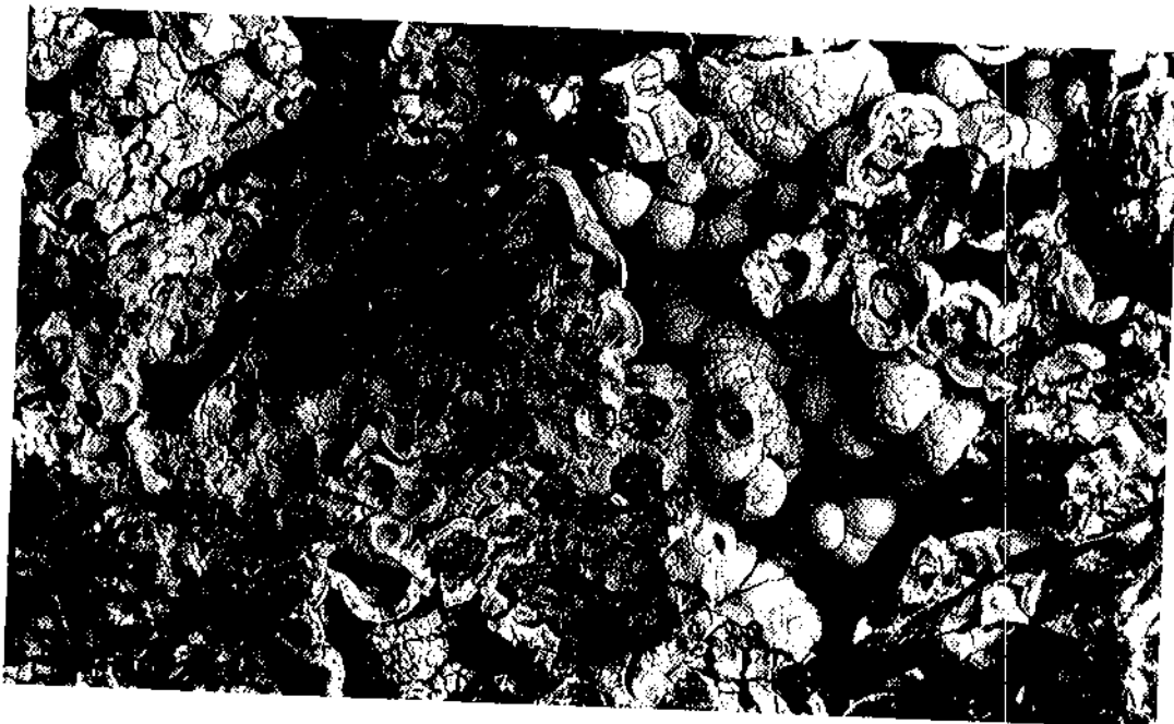
Figure 54. Back-scattered scanning electron micrograph (SEM 2816/4) of botroidal supergene pitchblende along a fissure in leucocratic phonolite (RFIII redox front; detail of Fig. 53).
