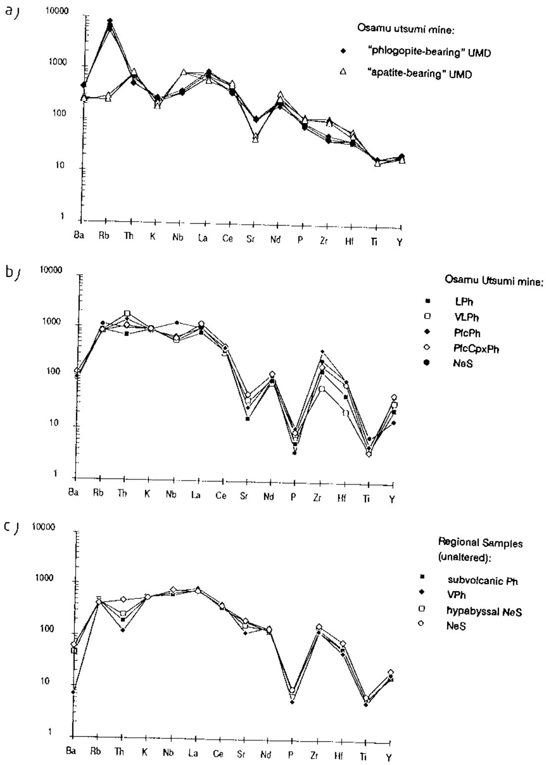
Figure 50. Incompatible elements normalised to chondrite and primitive mantle for: a) lamprophyric dykes from the Osamu Utsumi mine, b) average of hydrothermally altered rocks from the Osamu Utsumi uranium mine, c) unaltered regional rocks. (Normalisation factors from Thompson, 1983).
