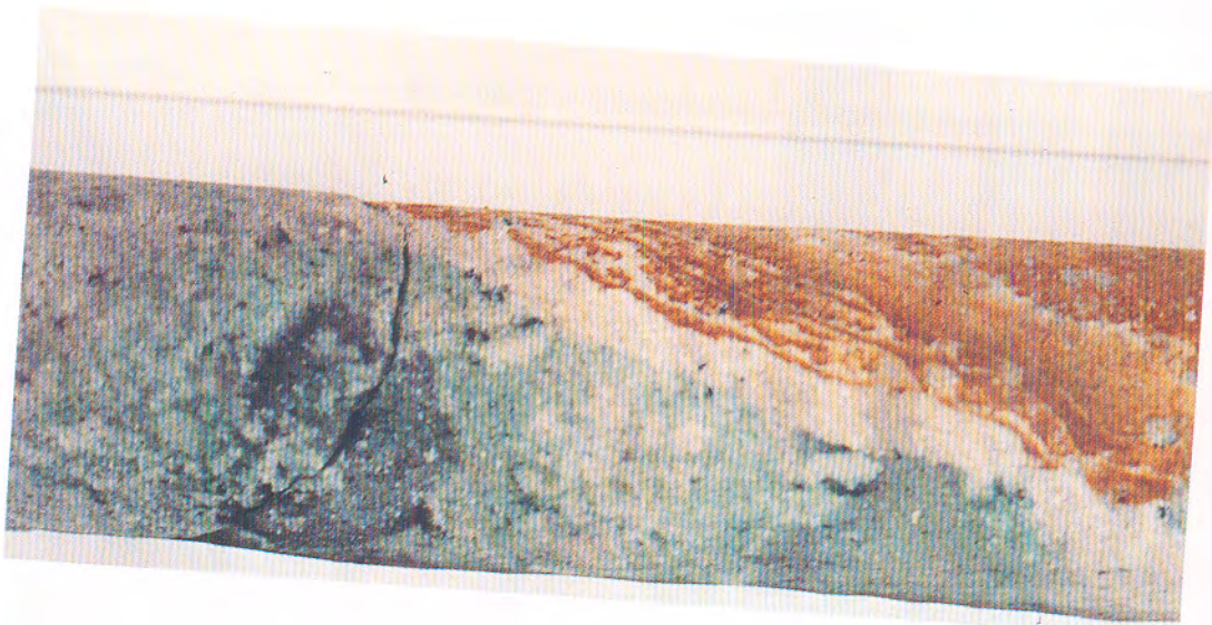
PLATE 3. Redox front at 33.5 m; drillcore F1.
