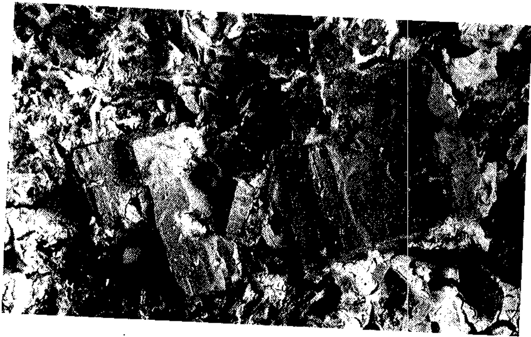
Figure 51. Back-scattered scanning electron micrograph of pyrite with pitchblende inclusions (SEM 2816/8); on the left side pitchblende is visible as bright inclusions. (Reduced leucocratic phonolite at 114 m from borehole F1).
