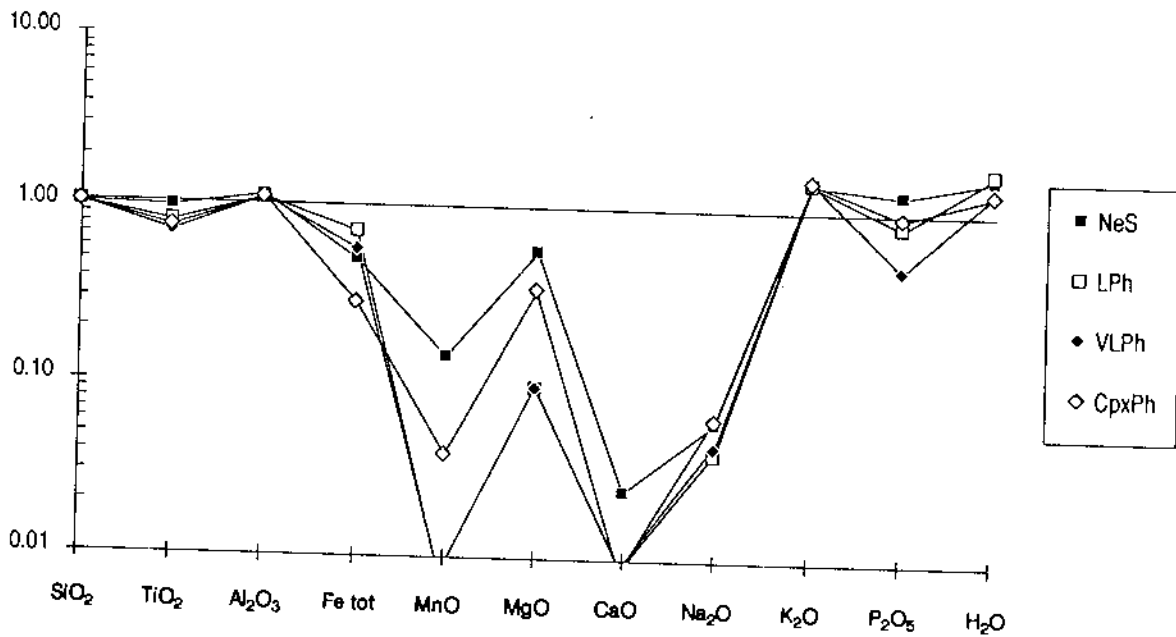
Figure 13. Average major element composition of hydrothermally altered, oxidised phonolites and nepheline syenites from the Osamu Utsumi mine normalised to the average composition of unaltered regional rocks.
