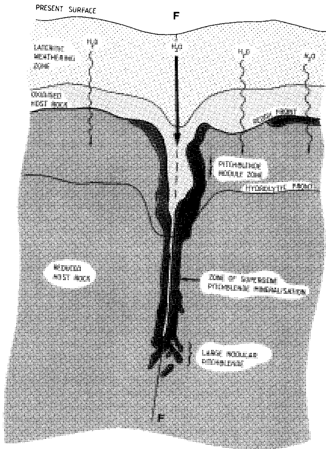
Figure 2. Schematic cross-section from the Osamu Utsumi mine showing the sequence of oxidation with depth, accompanied by supergene uranium mineralisation along the redox front and at greater depths marginal to the conductive fracture zone (F). (After Urânio do Brasil; unpublished report).
