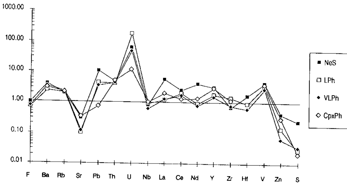
Figure 14. Average trace element composition of hydrothermally altered, oxidised phonolites and nepheline syenites from the Osamu Utsumi mine normalised to the average composition of unaltered regional rocks.
