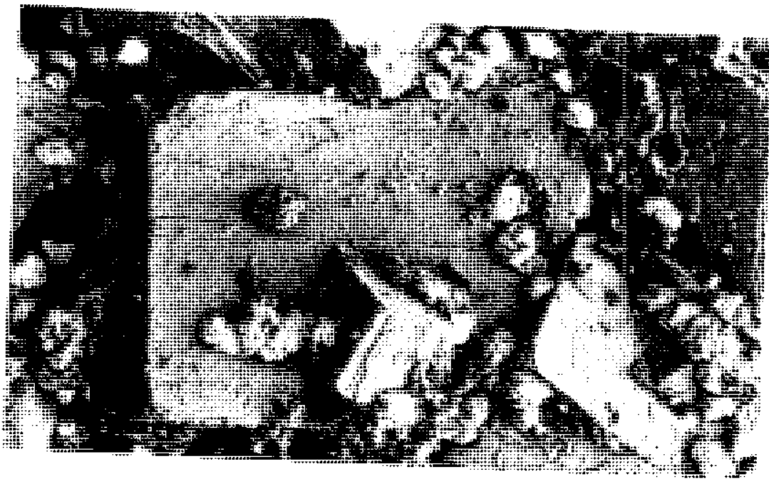
Figure 52. Scanning electron micrograph (SEM 2814/4) of idiomorphic monazites on pyrite. (Reduced leucocratic phonolite at 111 m from borehole F1).
