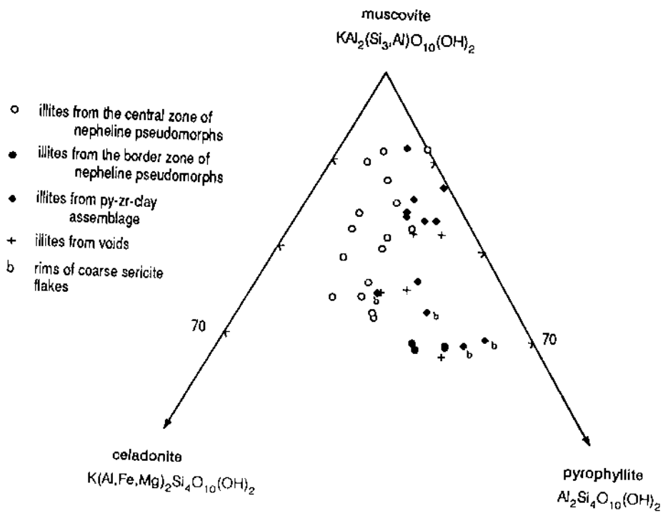
Figure 5. Compositional diagram of illites in different phonolitic rocks from the Osamu Utsumi mine with muscovite, celadonite and pyrophyllite as end members.
