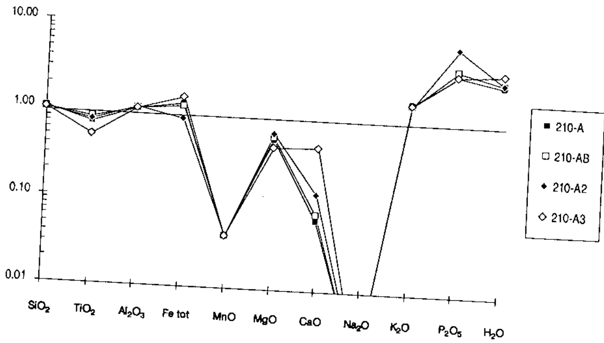
Figure 29. Major element compositions of the highly mineralised breccias at 210 m from borehole F4 normalised to the average composition of unaltered regional samples.
