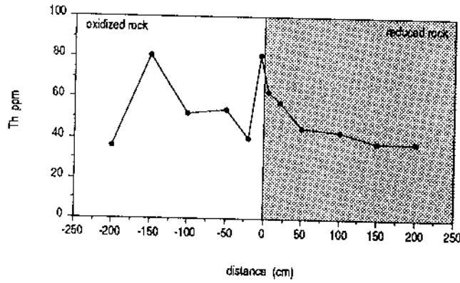
Redox Front RFII
