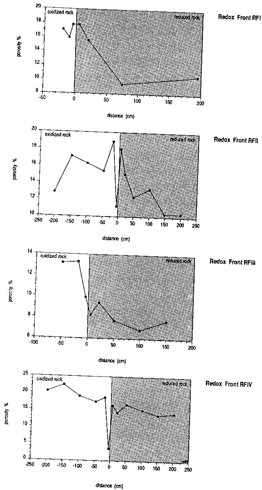
Figure 58. Variation of total porosity across the redox fronts. RFI from a mineralised dense phonolite; RFII from a breccia; RFIII from a dense leucocratic phonolite; RFIV from a porous cpx-bearing phonolite.
