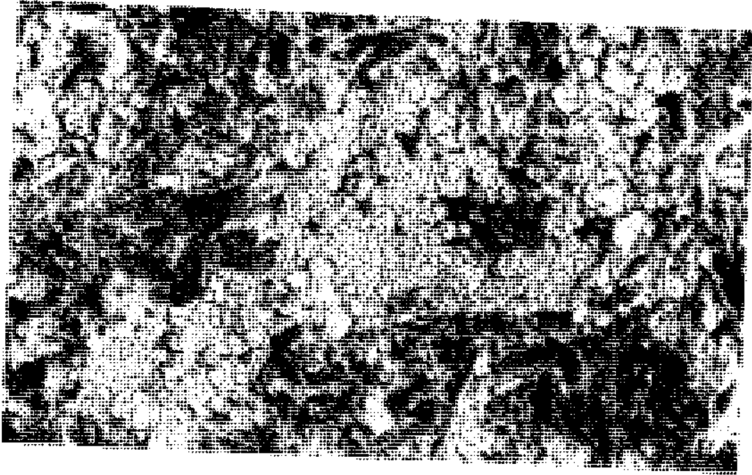
Figure 53. Back-scattered scanning electron micrograph (SEM 2815/10) of botroidal supergene pitchblende along a fissure in leucocratic phonolite (RFIII redox front).
