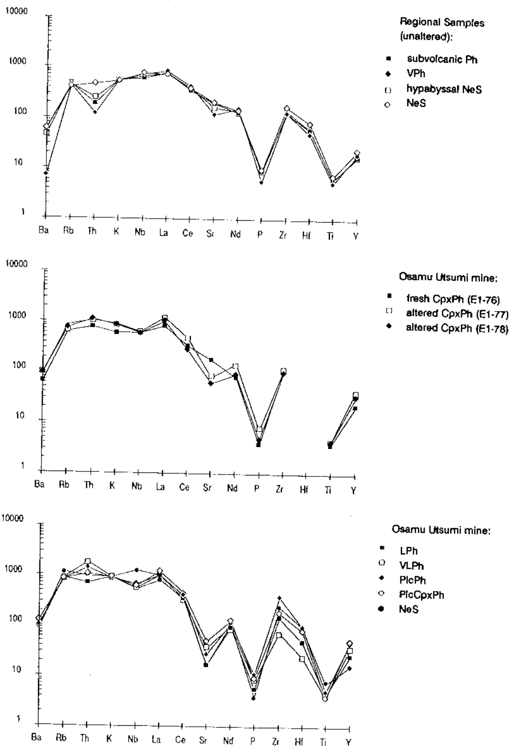
Figure 12. Incompatible elements normalised to chondrite and primitive mantle for:
