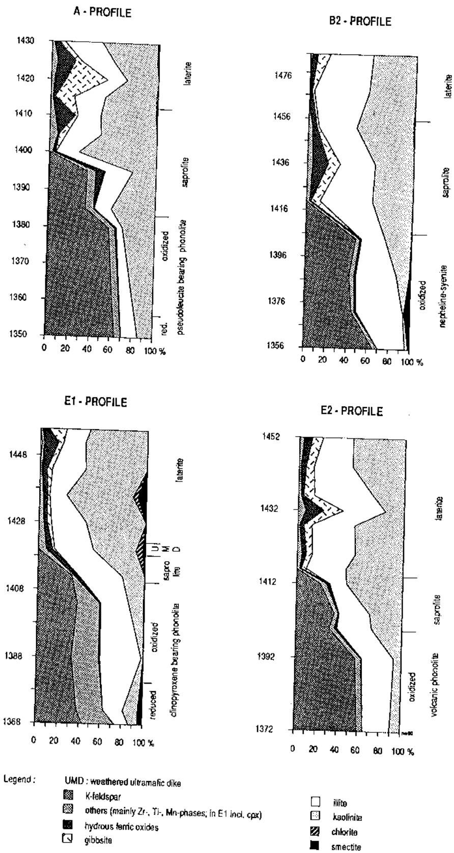
Figure 7. Mineralogical compositions in four weathering profiles from different parent rocks. Profile locations are indicated in Figure 4.
