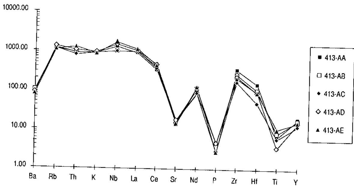
Figure 24. Incompatible elements normalised to chondrite and primitive mantle for hydrothermally altered, reduced nepheline syenite xenolith at 413 m depth from borehole F4, (normalisation factors from Thompson, 1982).
