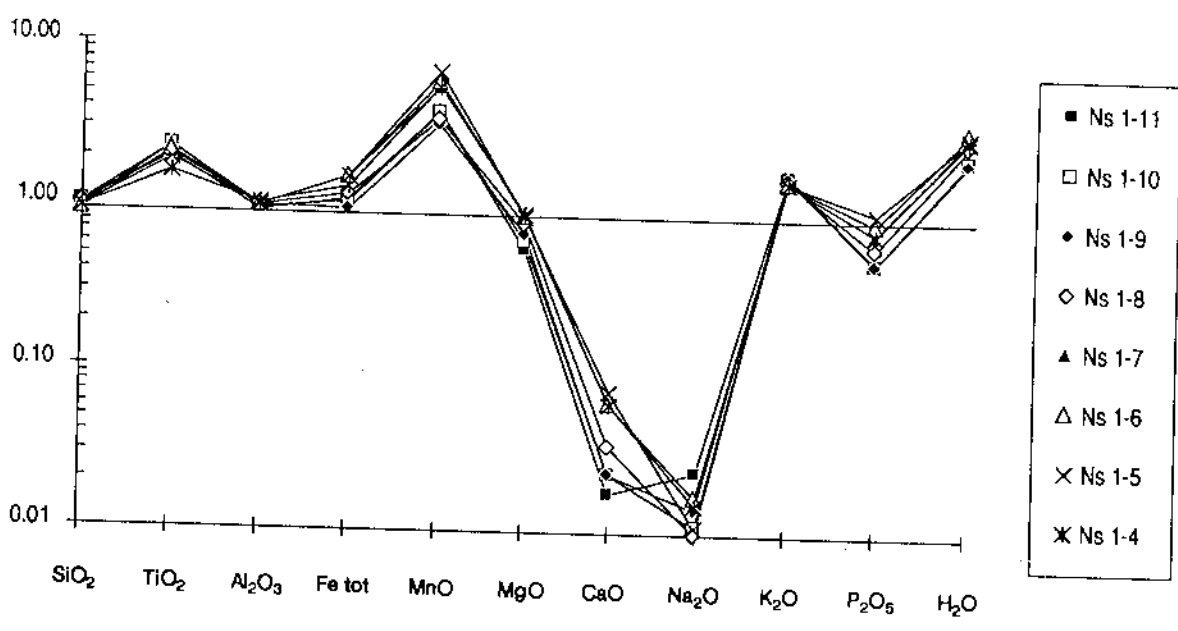
Figure 18. Average major element composition of a hydrothermally altered, reduced nepheline syenite xenolith at 353 m depth from borehole F4, normalised to the average composition of unaltered regional rocks.
