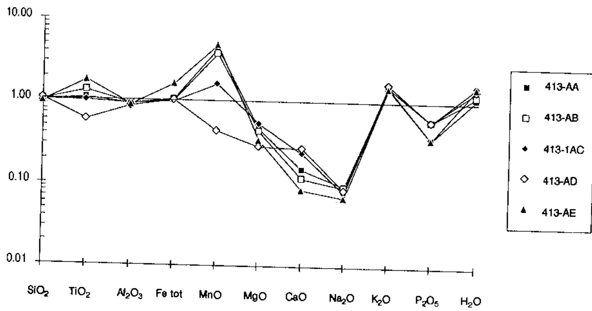
Figure 19. Average major element composition of hydrothermally altered, reduced nepheline syenite xenolith at 413 m depth from borehole F4, normalised to the average composition of unaltered regional rocks.
