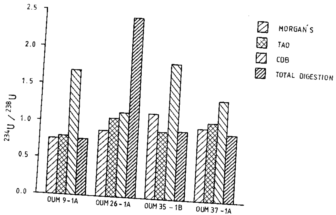
Figure 2-2. 234 U/ 238 U activity ratios for particular phases, characterised by extraction by particular reagents.
