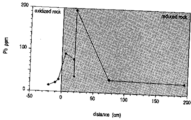
Redox Front RFI
