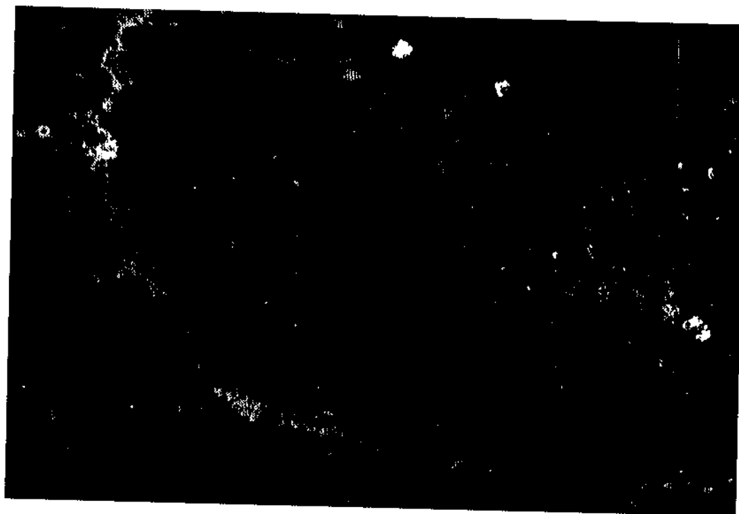
PLATE 6:1-8. Cathodoluminescence image of (two quarters of) a pitchblende nodule of total maximum diameter about 10 mm from a redox front in fine-grained phonolite. Note the non-emission of pitchblende impregnated (dark to black) portions of the nodule and the light yellowish-reddish emission of the illite - K-feldspar - kaolinite silicate mineral matrix of the nodule after pitchblende dissolution along the borders and in the left-hand part of the nodule (seen only in the upper photograph). Open pores in the nodule show light-blue or dark-(ink) blue emission (depending on the presence of preparation adhesives covering the glass support of the polished rock thin section) and dark- (ink) blue emission, if within the surrounding silicate matrix of the nodule (which was better impregnated by the preparation adhesives). The emission colours of the surrounding rock matrix are medium yellowish-grey and the finely disseminated black minerals are non-emitting (mostly submillimetric) pyrites. Compare with same nodule in plain light view (PLATE 6:1-9).
