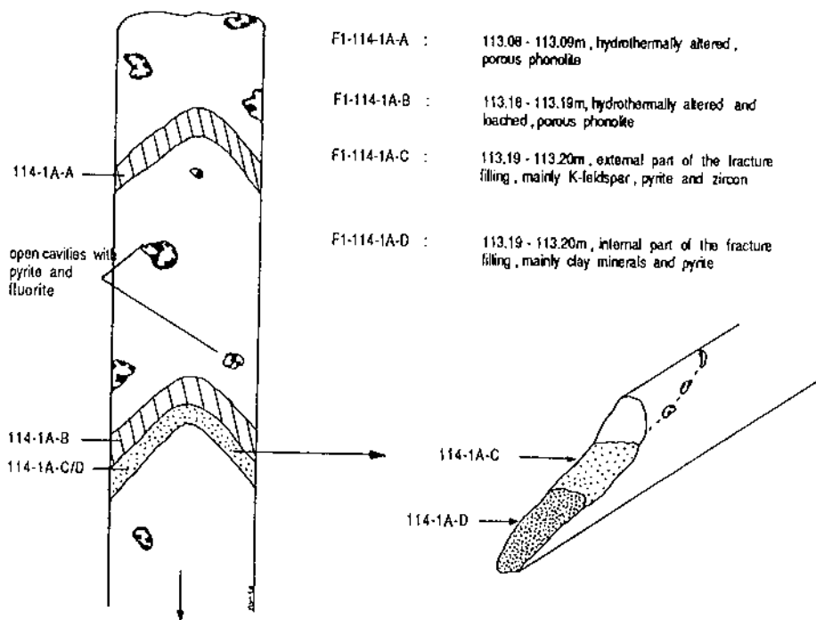
Figure 46. Conductive fracture in drillcore F1 at a depth of 113 m; sample location is indicated by the hatched areas.
