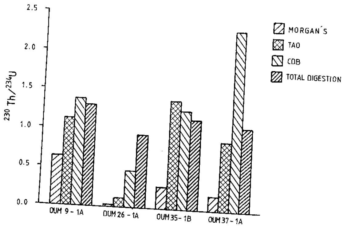
Figure 2-3. ^{230}\text{Th}/^{234}\text{U} activity ratios for particular phases, characterised by extraction by particular reagents.
