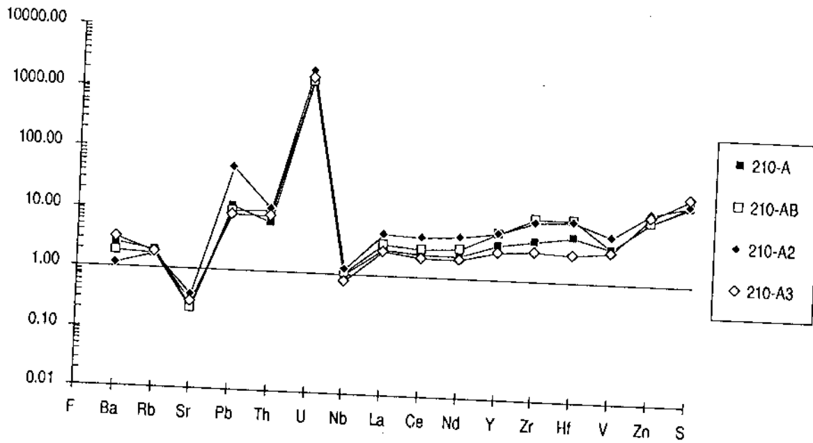
Figure 33. Trace element compositions of the highly mineralised breccias at 210 m from borehole F4 normalised to the average composition of unaltered regional samples.
