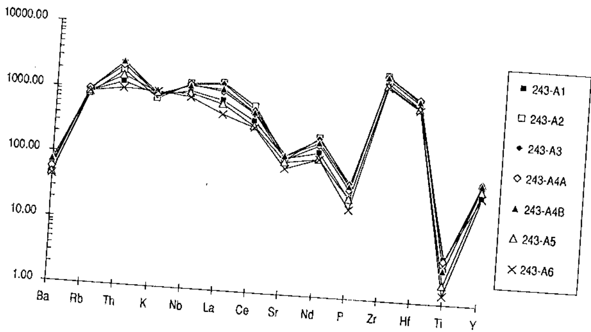
Figure 38. Incompatible elements normalised to chondrite and primitive mantle of the highly mineralised breccias at 243 m from borehole F4 (normalisation factors from Thompson, 1982).
