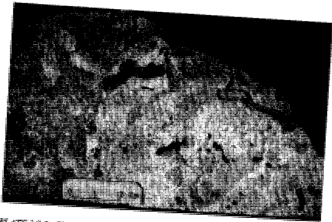
PLATE 3.9-5. Phonolite with redox front. Note the forms of the pitchblende nodules on the natural fracture plane and the incipient dissolution of the nodules near the redox front; these nodules change colour from black to medium-grey. Open pit sample no.: S/N 21 (8-2 AH 63).
